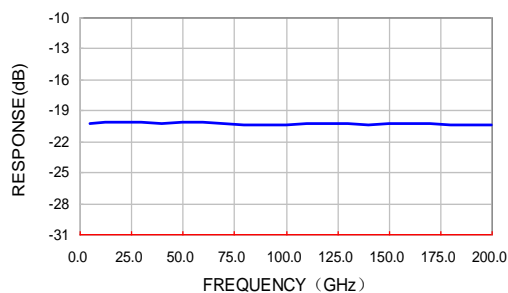
at +12V Pin= -20dBm — S12
