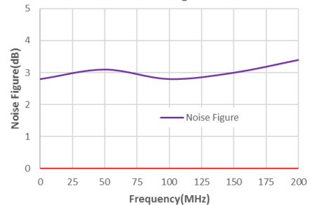
Noise Figure
