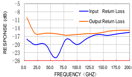
at +12V Pin= -20dBm
